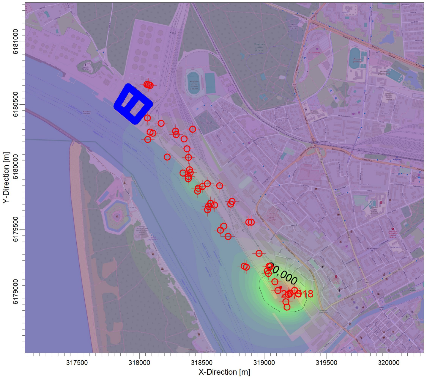
PLOT FILE OF PERIOD VALUES AVERAGED ACROSS 5 YEARS FOR SOURCE GROUP: ALL ug/m 3
